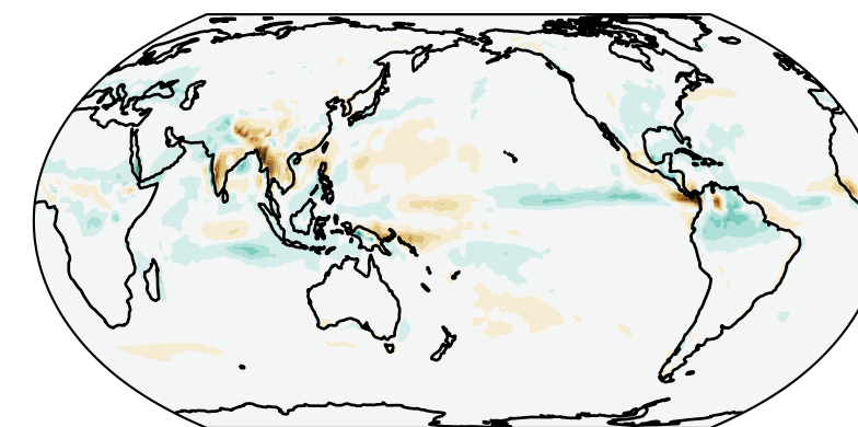
Precipitation rate (JJA) EAMv3 - EAMv2
