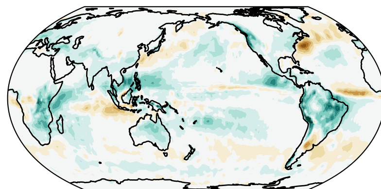
Precipitation rate (DJF) EAMv3 - GPCP
