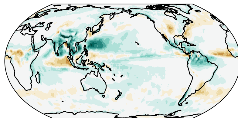
Precipitation rate (JJA) EAMv3 - GPCP
