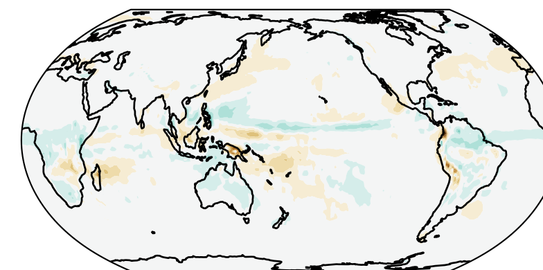
Precipitation rate (DJF) EAMv3 - EAMv2
