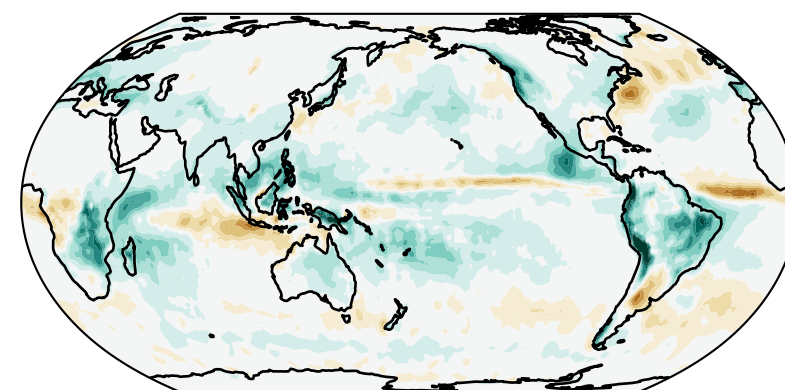
Precipitation rate (DJF) EAMv2 - GPCP
