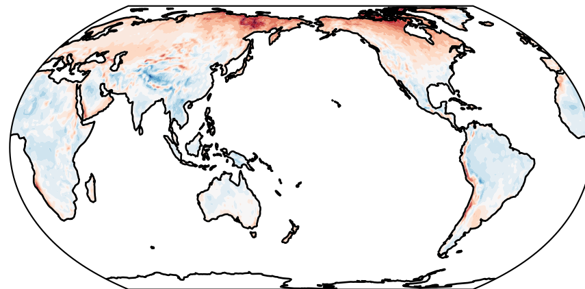
2-m Air Temperature EAMv2 - CRU
