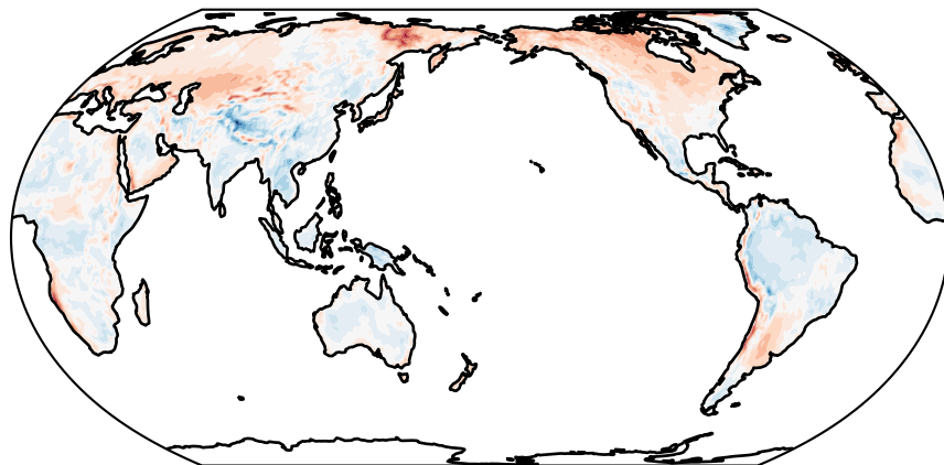
2-m Air Temperature EAMv3 - CRU
