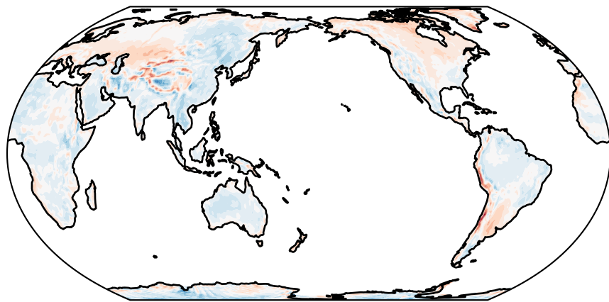
2-m Air Temperature: EAMv3 - ERA5 (Bias: -0.36 K / RMSE: 1.94 K/ r : 0.99)
