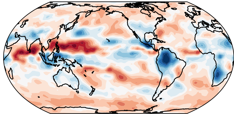
Longwave Cloud Feedback
