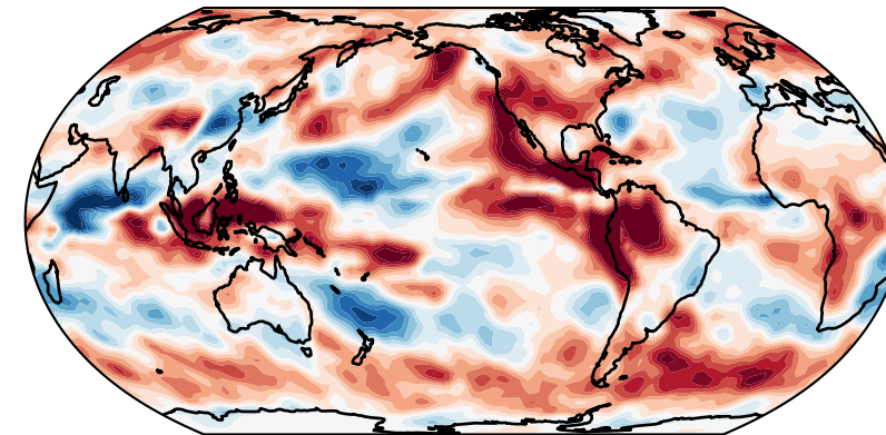
CMIP5/6 Ensemble Mean Shortwave Cloud Feedback Difference
