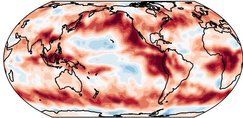
Net Cloud Feedback
