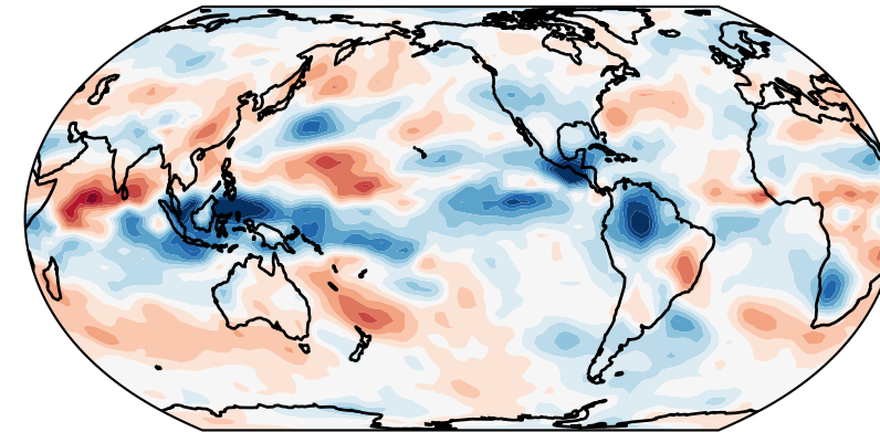
Longwave Cloud Feedback Difference
