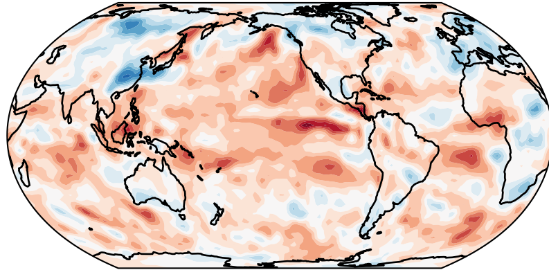
Net Cloud Feedback Difference
