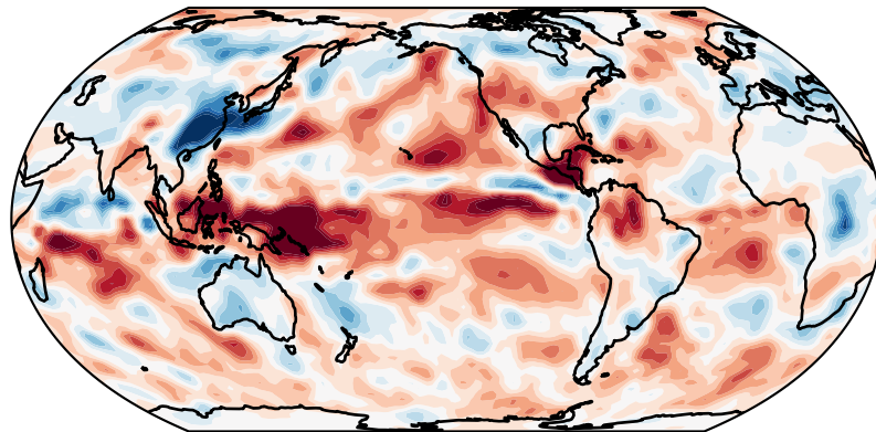
12km SCREAM Ensemble Mean Shortwave Cloud Feedback Difference
