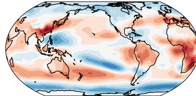
CMIP5/6 Ensemble Mean Shortwave Cloud Feedback
