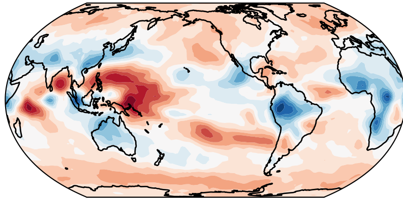
Longwave Cloud Feedback
