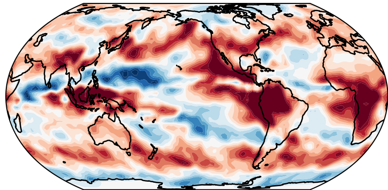
SCREAM 3km Shortwave Cloud Feedback
