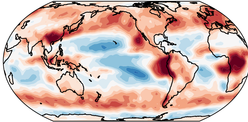
Net Cloud Feedback
