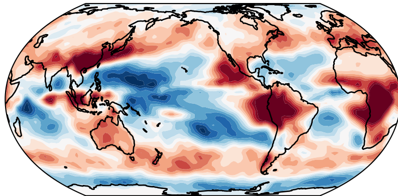
SCREAM 12km Ensemble Mean Shortwave Cloud Feedback
