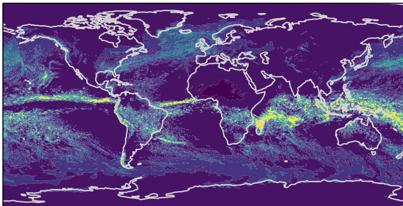
SCREAMv1 (3.28 mm/day)
