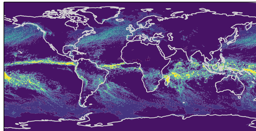
SCREAMv0 (3.15 mm/day)
