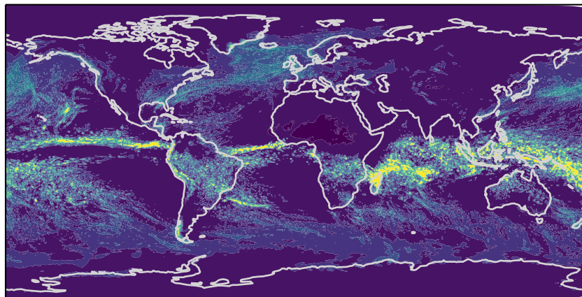
EAMxx (3.28 mm/day)
