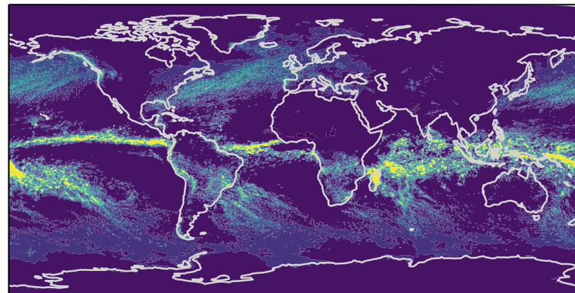
EAMf90 (3.15 mm/day)
