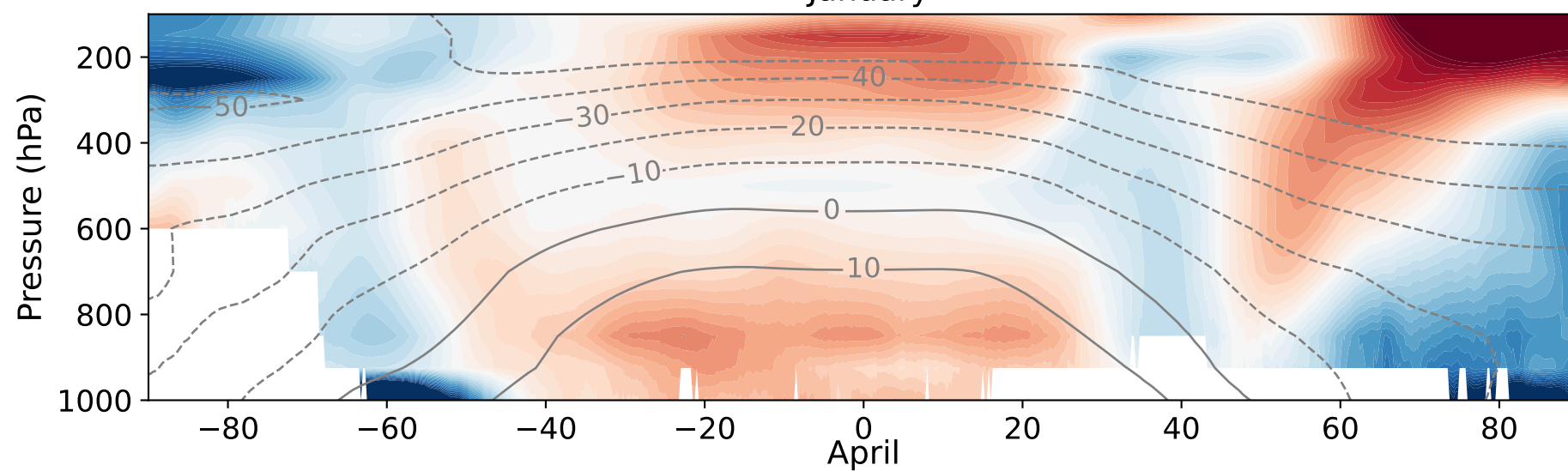
SCREAMv1 minus ERA5 temperature difference January
