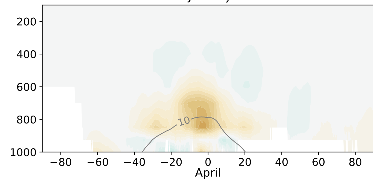
SCREAMv1 minus ERA5 humidity difference January
