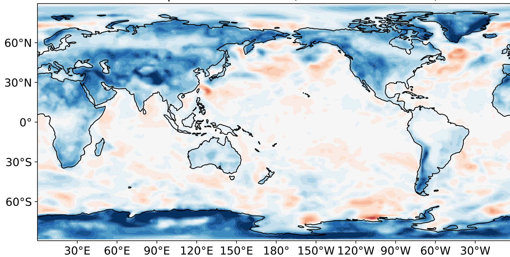
2-m temperature difference (TMS minus v1 default)
