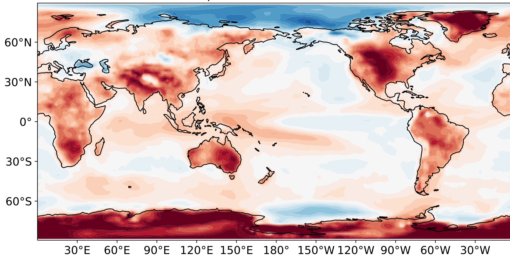
2-m temperature bias (v1 minus ERA5)
