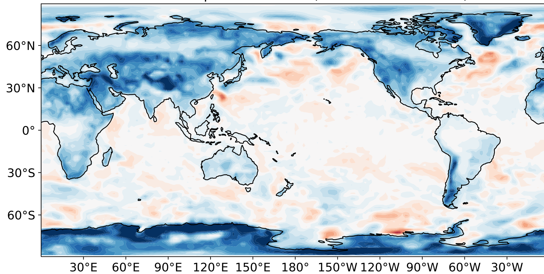
10-m wind speed difference (TMS minus v1 default)
