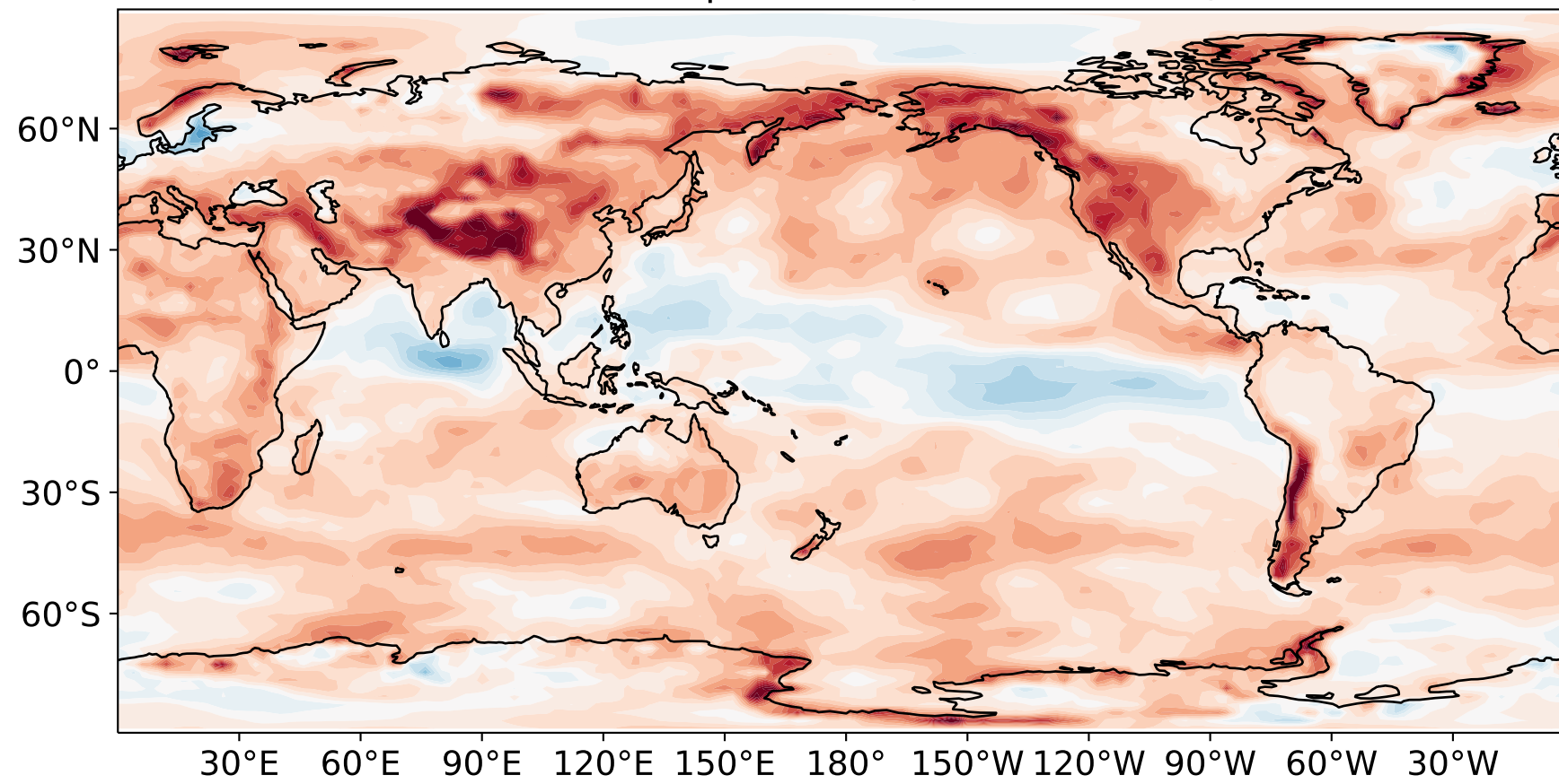
10-m wind speed bias (v1 minus ERA5)
