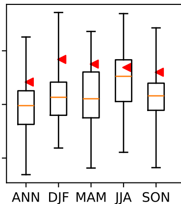
(i) Zg-500 (hm)
