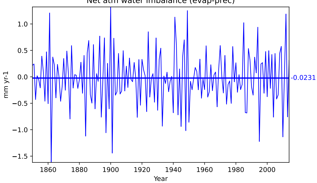
Net atm water imbalance (evap-prec)
