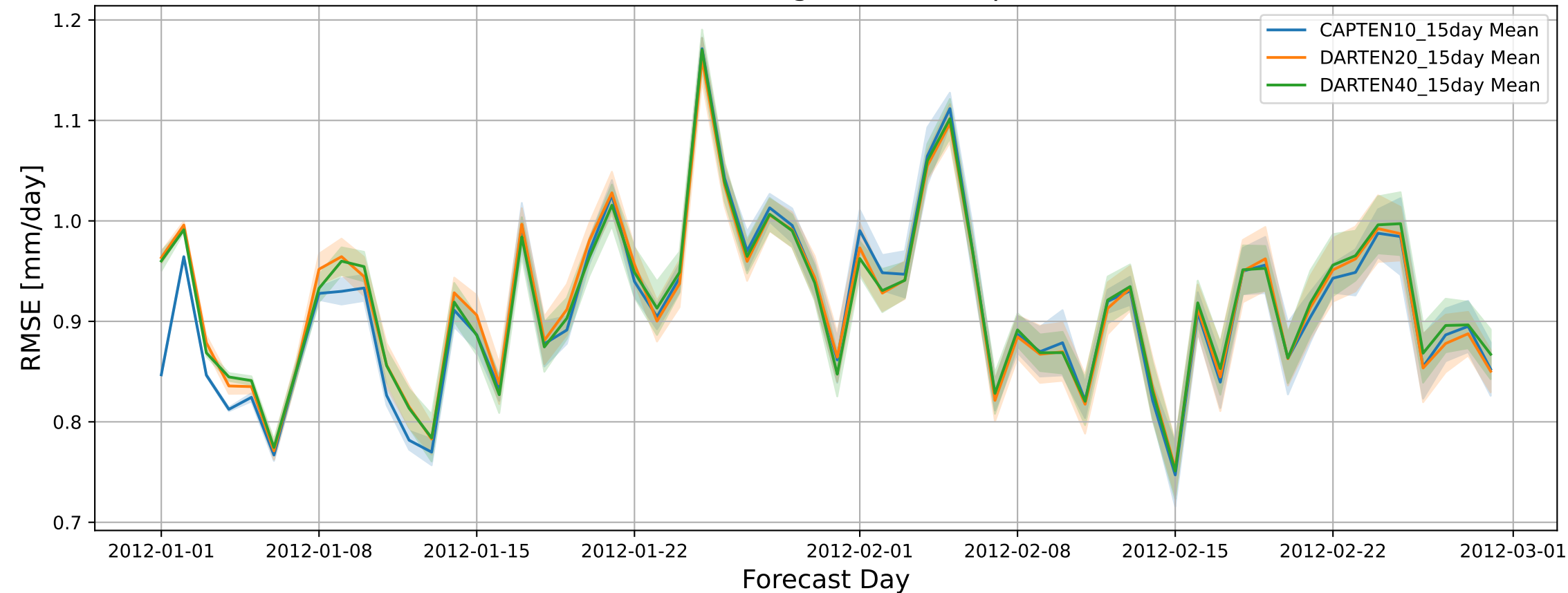
Time-Evolving RMSE in Tropics
