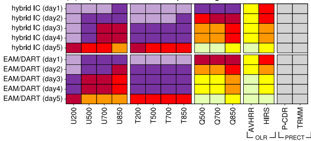
(a) Spatial correlation, polar regions
