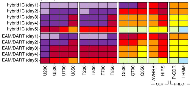
(c) Spatial correlation, mid-latitudes
