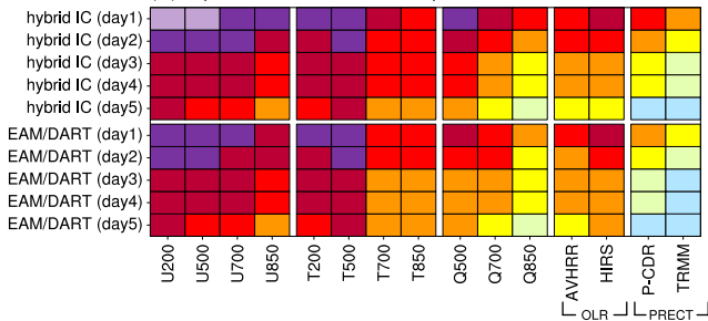
(e) Spatial correlation, tropics
