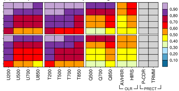
(b) Temporal correlation, polar regions
