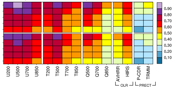
(f) Temporal correlation, tropics
