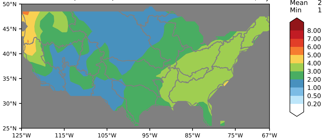
LRv1-Transient (1950-1969)
