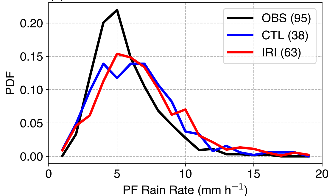
(c) MCS PF Mean Rain Rate
