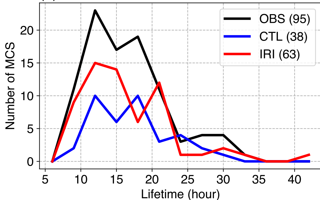
(a) MCS Lifetime
