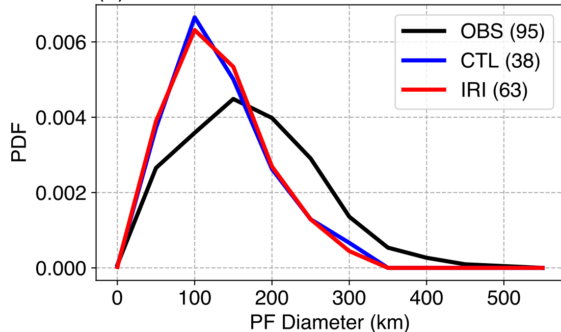
(b) MCS PF Diameter
