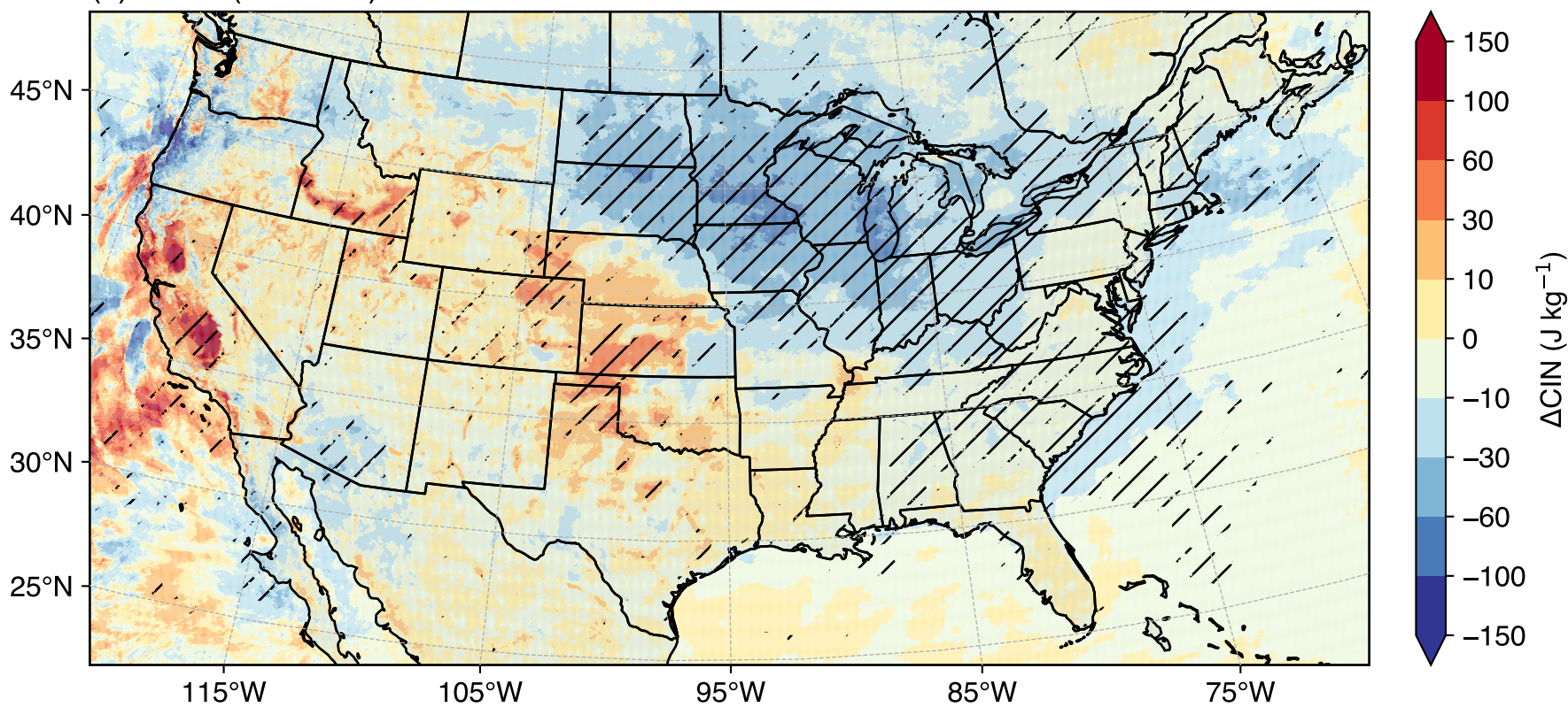
(c) \Delta\text{CIN} (11-14LT)
