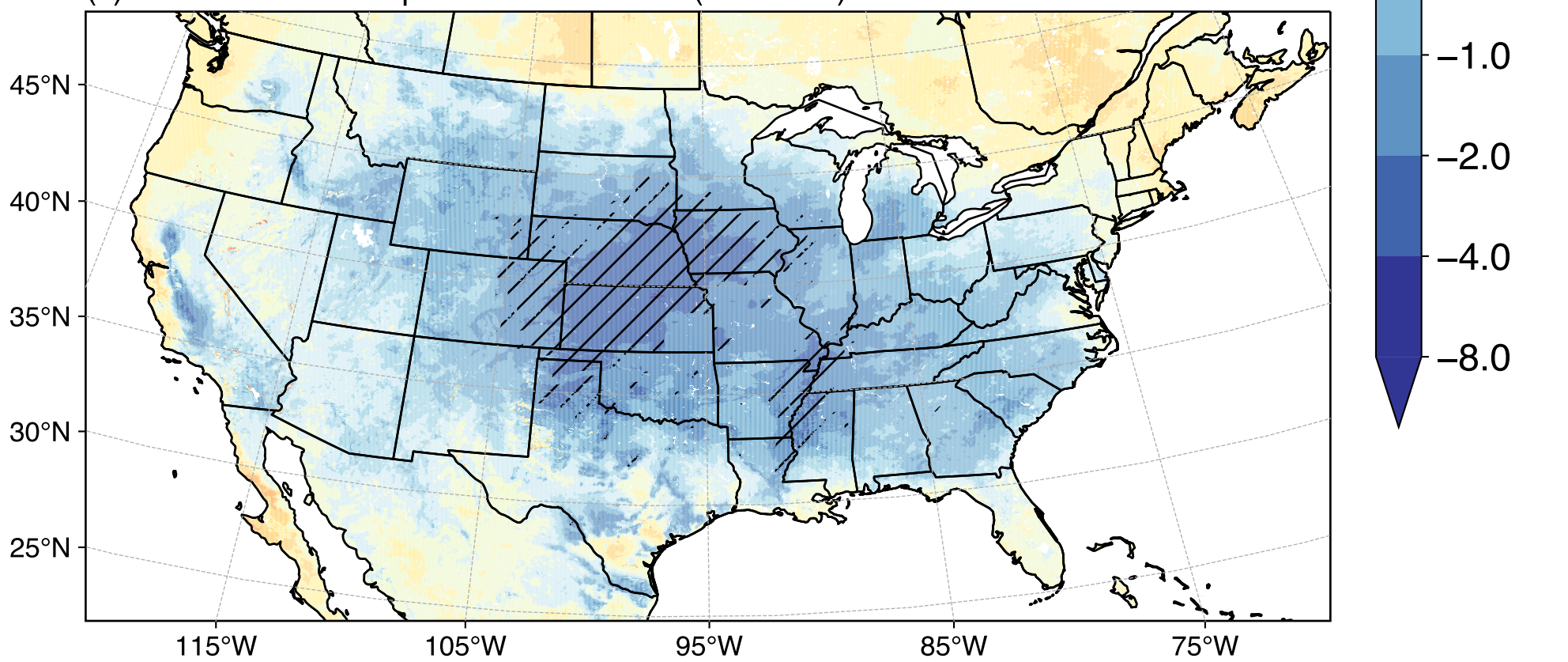
(c) WRF JJA 2m Temperature Difference (IRI - CTL)
