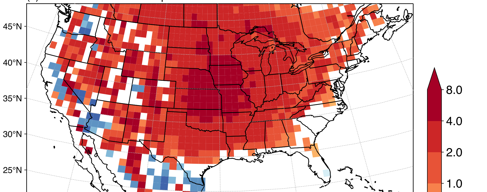
(b) WRF JJA 2m Temperature Bias (CTL - PRISM)
