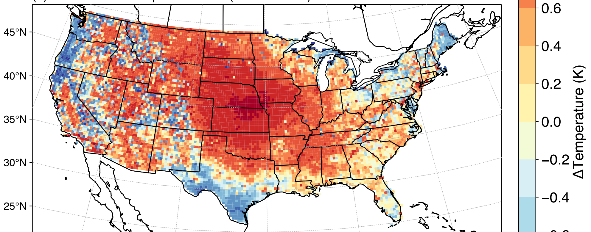
(c) WRF JJA 2m Temperature Difference (IRI - CTL)
