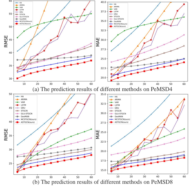
Figure 6: Performance changes of different methods as the forecasting interval increases.
