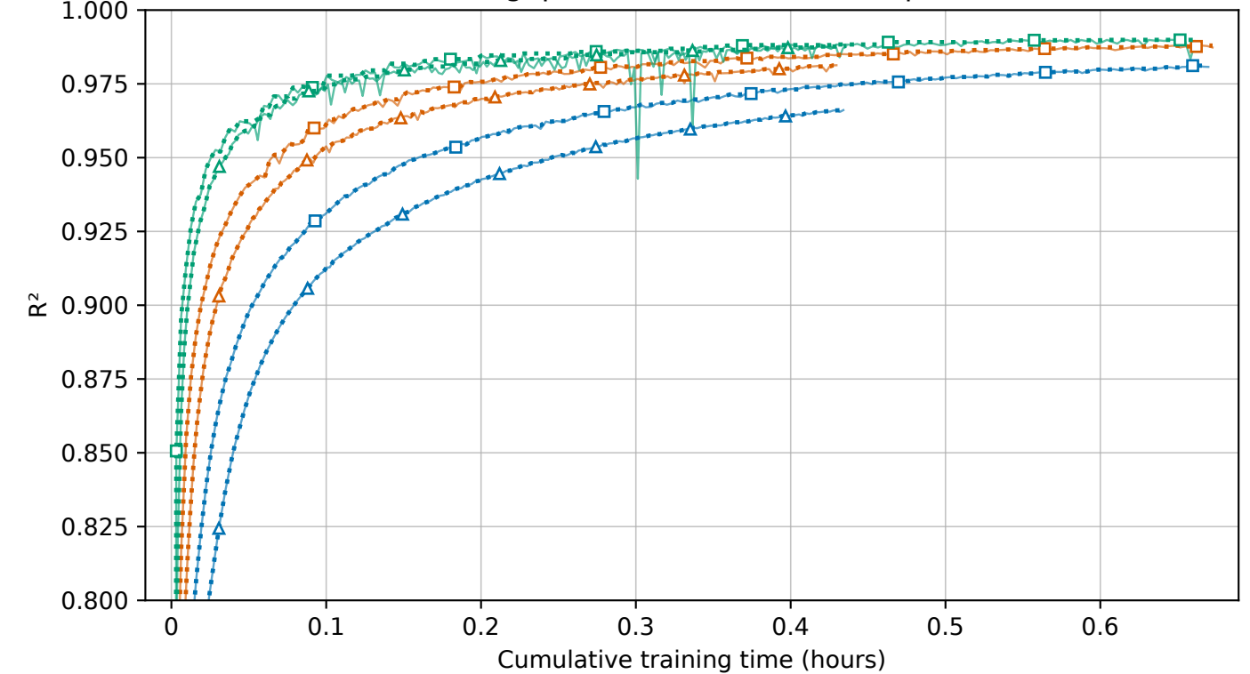
Training: pooled R 2 in normalized space
