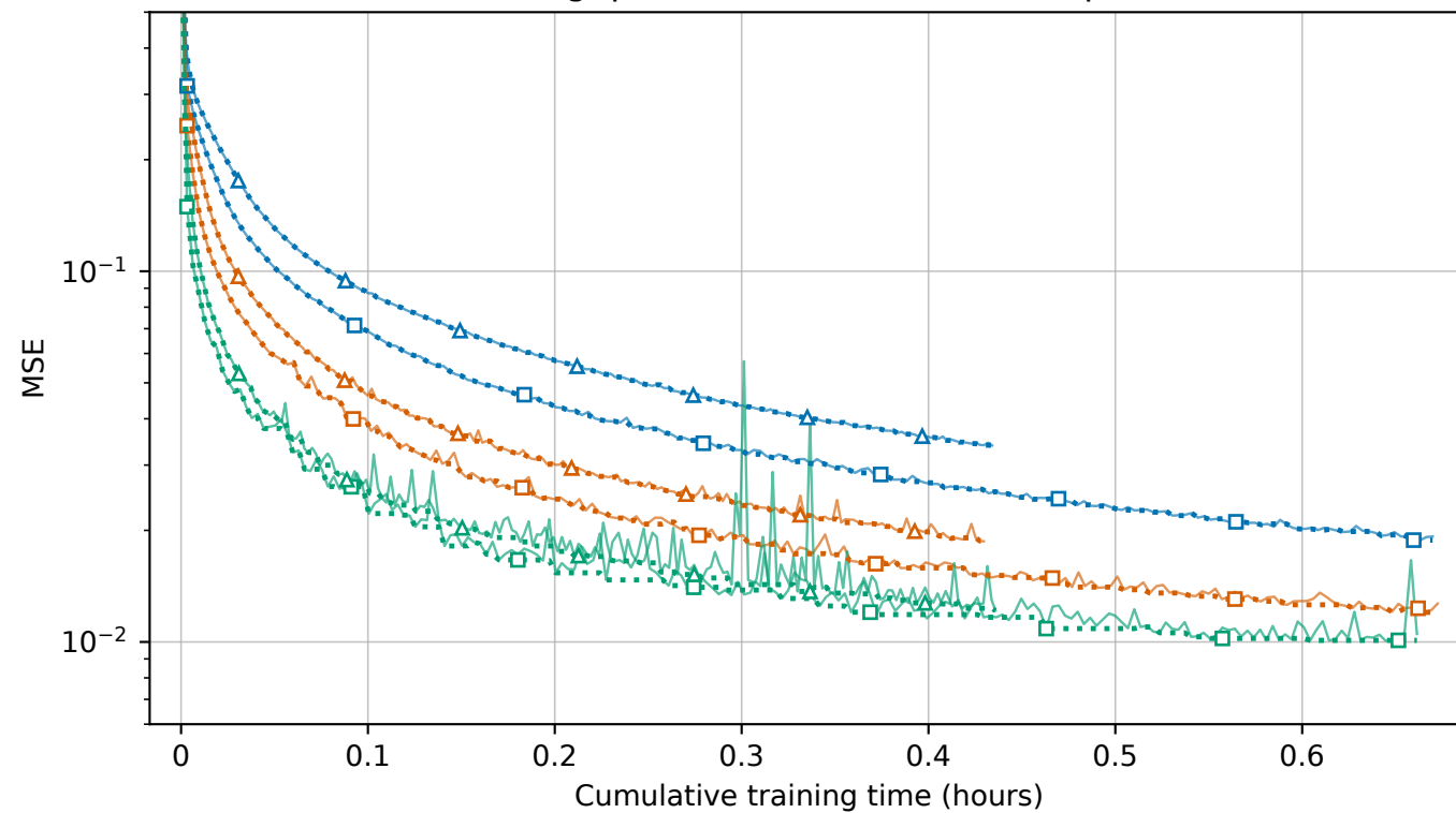
Training: pooled MSE in normalized space
