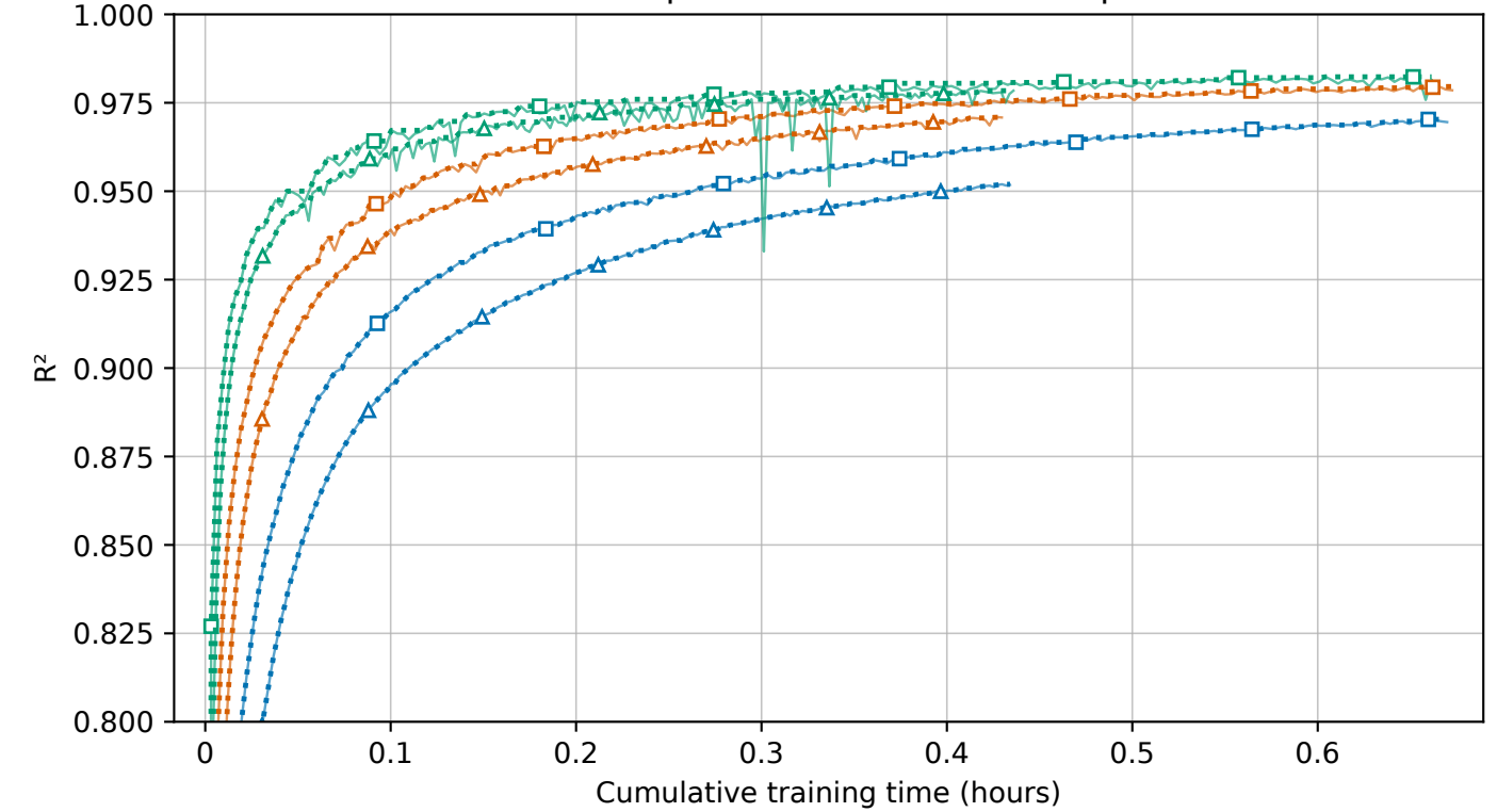
Validation: pooled R 2 in normalized space
