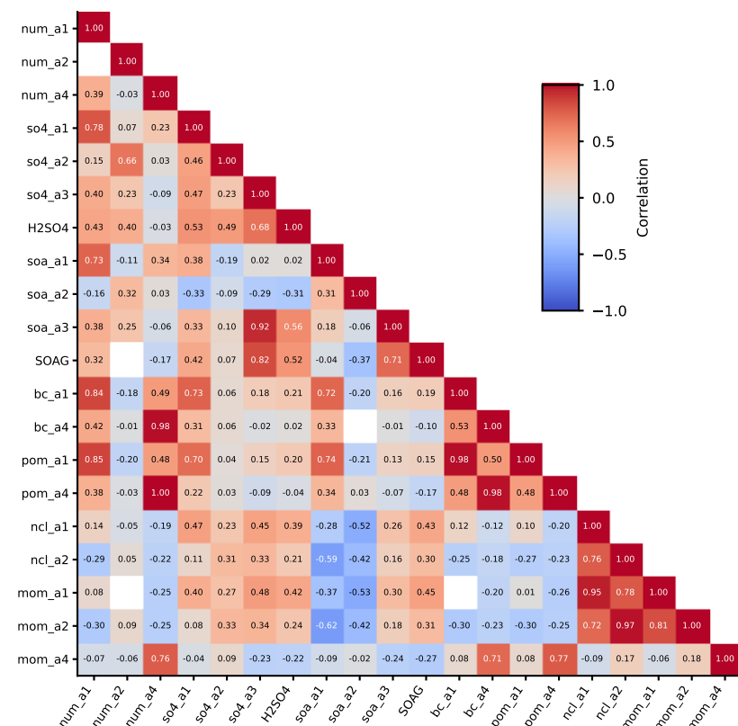
Pearson after Symmetric log
