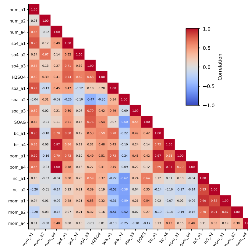
Pearson after Power 1/3
