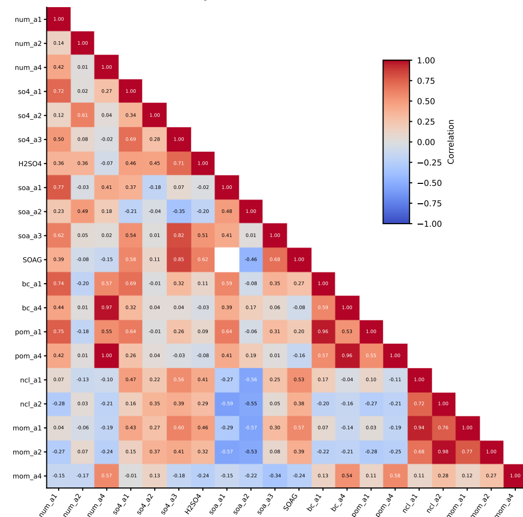
Spearman rank correlation
