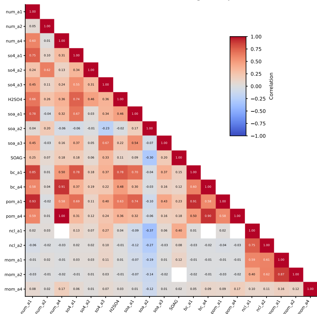
Pearson correlation: original inputs
