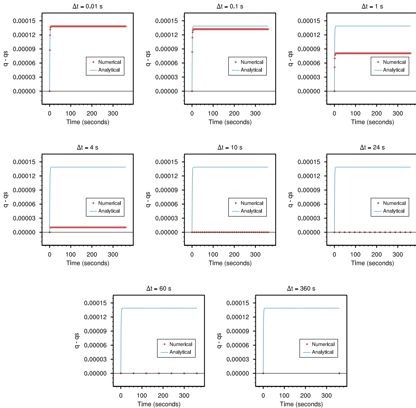
Time evolution of q - q_s ( \tau_1 = 3600 s, \tau_2 = 1 s)
