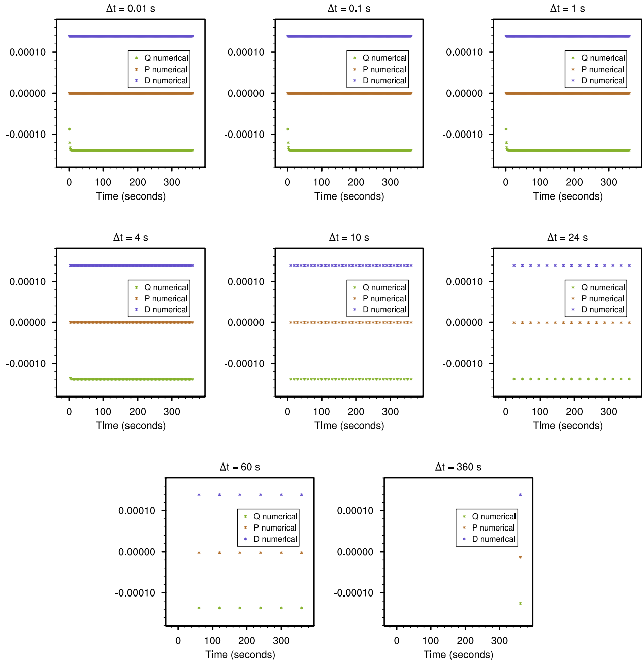
D, P, and Q time series ( \tau_1 = 3600 s, \tau_2 = 1 s)
