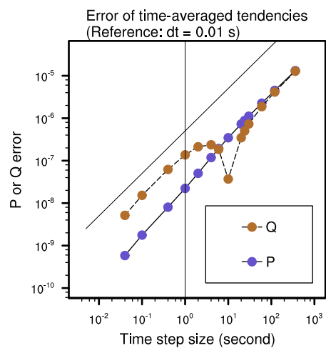
Convergence diagrams for state and tendencies ( \tau_1 = 3600 s, \tau_2 = 1 s)
