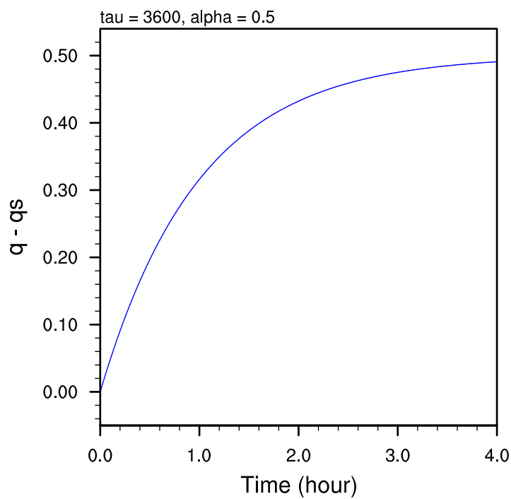
Analytical solution of the D+P problem
