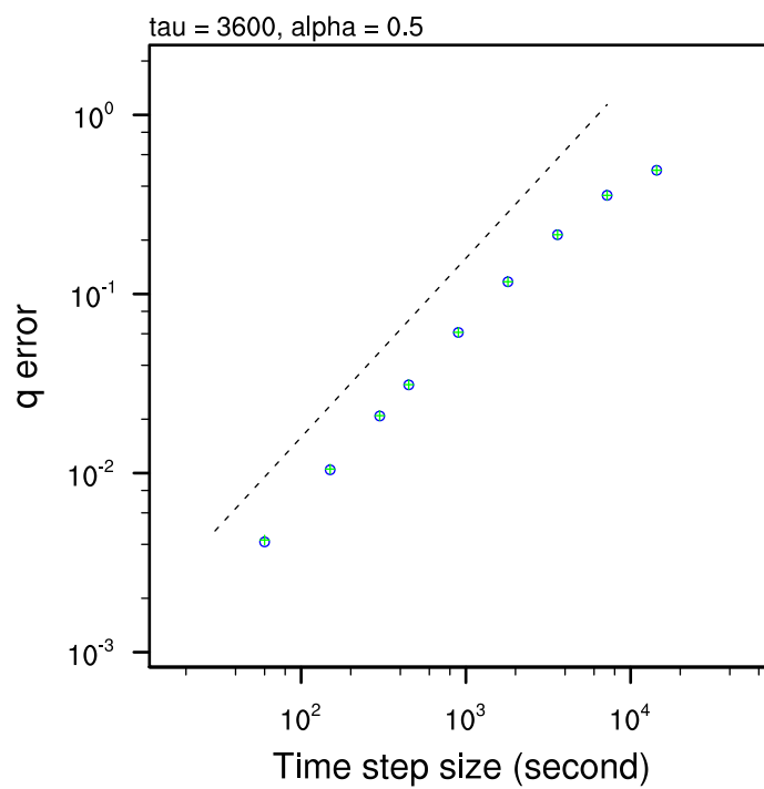
Solution error at 4 hours
