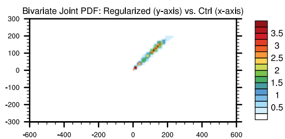
LHF (ocean only)
