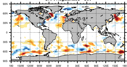
SHF: Regularized - Ctrl
