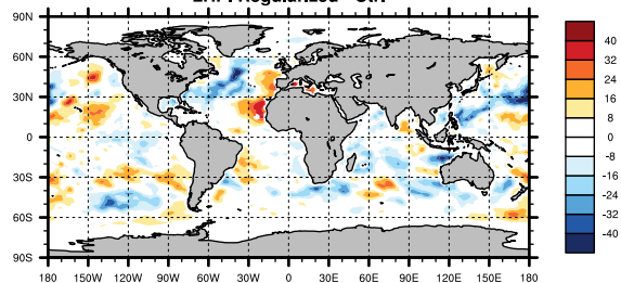
LHF: Regularized - Ctrl
