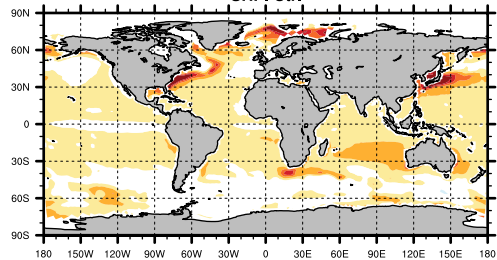
SHF: Ctrl
