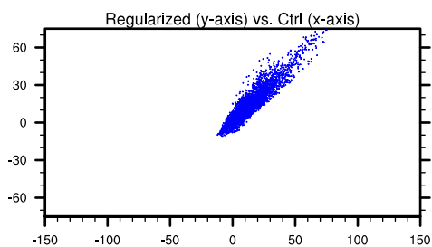
SHF (ocean only)
