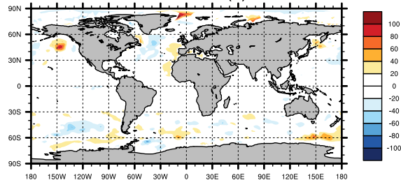
LHF: Relative diff. (%)
