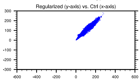
LHF (ocean only)
