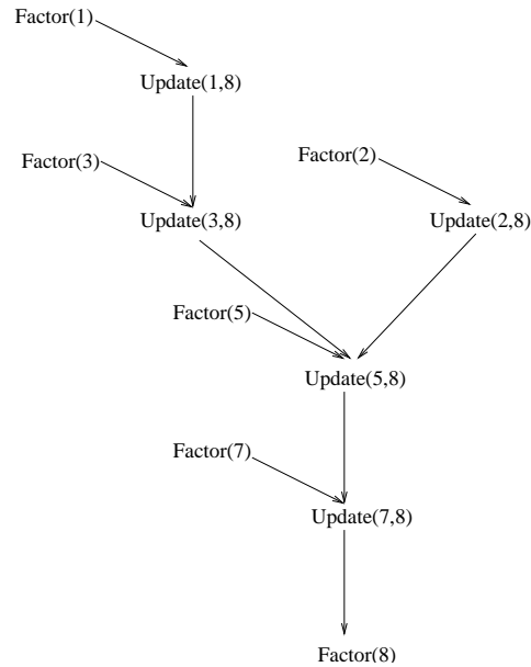
Figure 5: Illustration of several dependencies involved in the factorization of supernode 8 for the matrix in Figure 1
